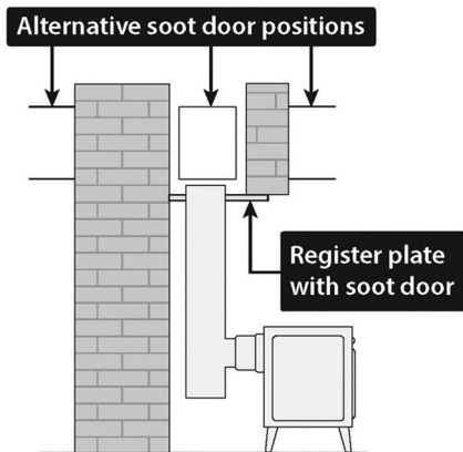
Horizontal register plate with rear flue connection
